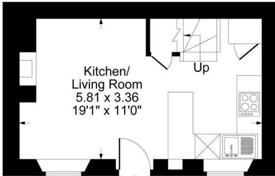
IN Ground Floor
